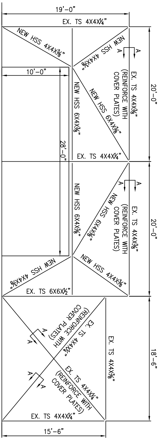
1 SHEAR WALL STRUCTURAL DETAIL
